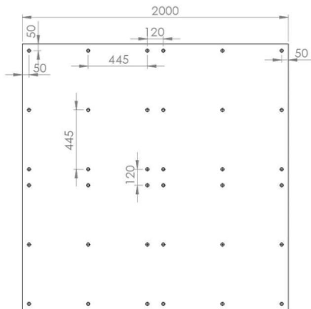
VISTA FRONTAL CHAPA FRONTAL
